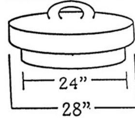
-Manhole Cover-
