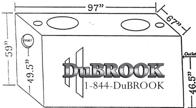
- 1000 Gallon Tank - 7,600 lbs. (2 Compartment - 8,000 lbs.)
