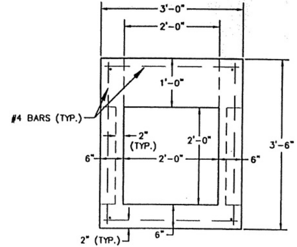
SIDE
