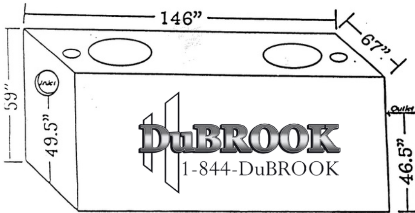
- 1500 Gallon Tank - 11,000 lbs. (2 Compartment - 11,500 lbs.)
